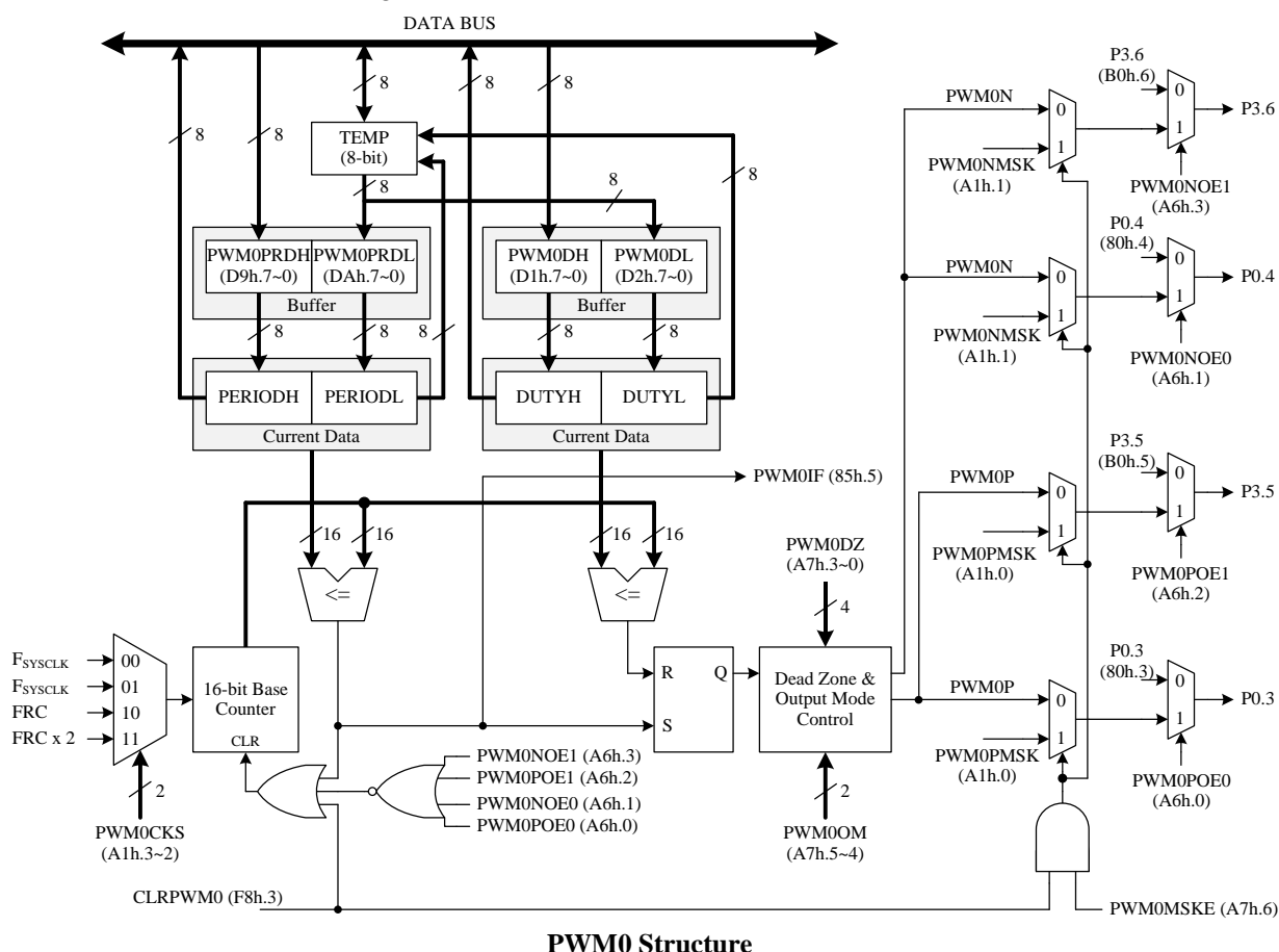
PWM0 Structure
